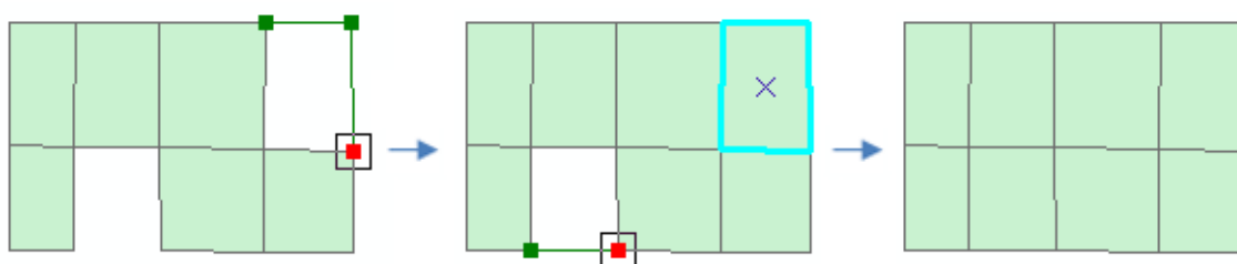
Figure 23. Autocomplete polygons
