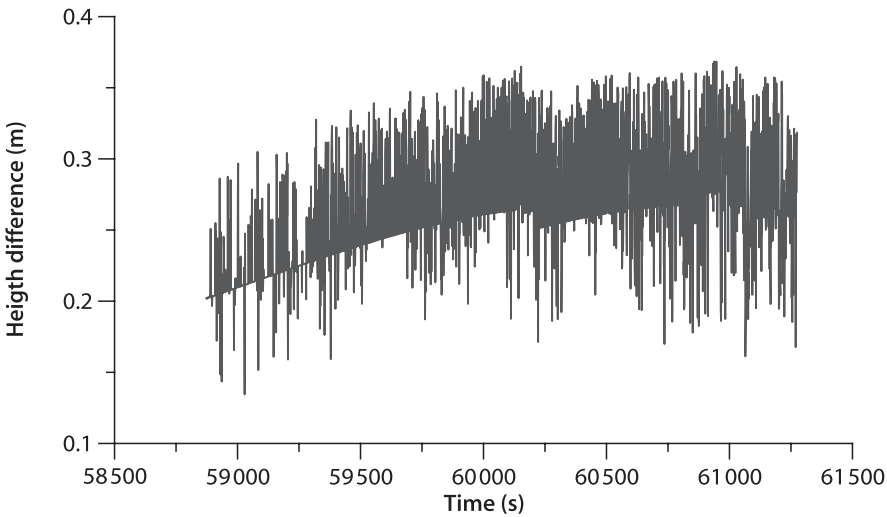
Fig. 10.14. Height differences caused by static references
