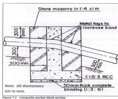
Figure 7.2 Composite anchor block section
