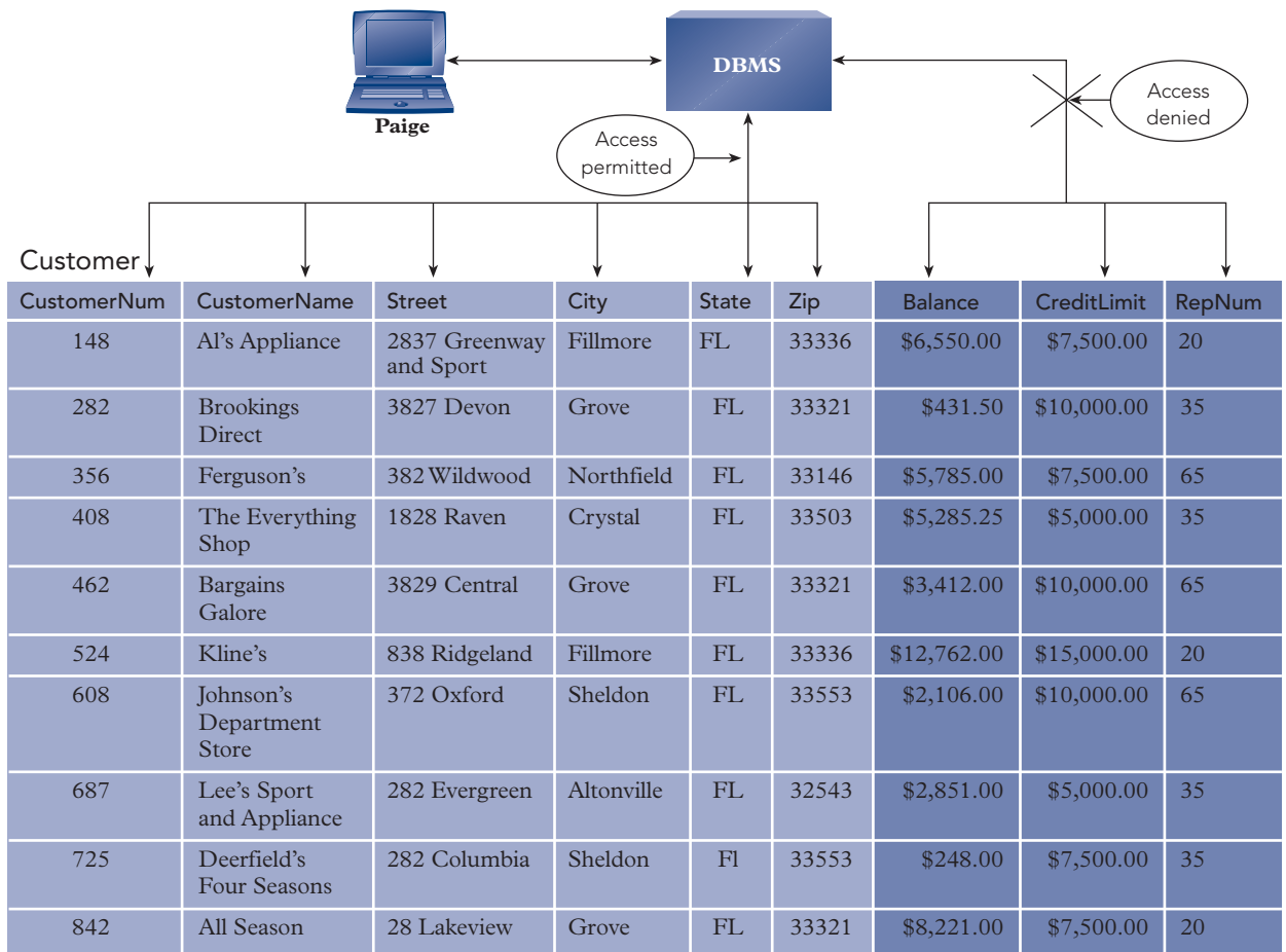
FIGURE 8-3 Permitted and denied access privileges for Paige
