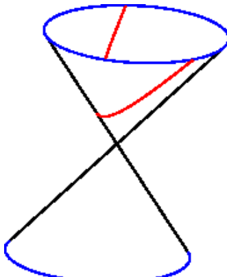
Parabolic: پارابول \beta = \alpha/2
