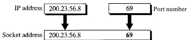
Figure 23.5 Socket address
