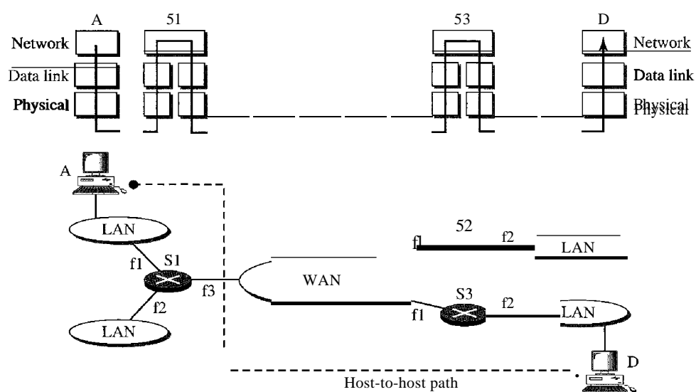
Figure 20.2 Network layer in an internetwork
