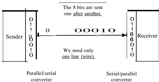
Figure 4.33 Serial transmission
