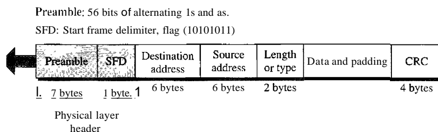
Figure 13.4 802.3 MAC frame
