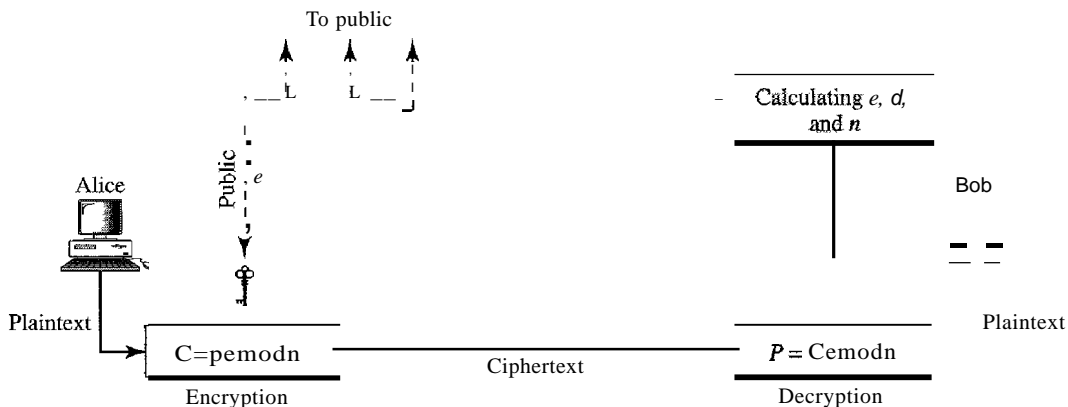
Figure 30.24 RSA
