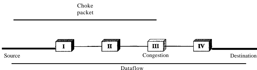
Figure 24.7 Choke packet
