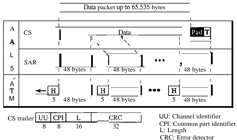
Figure 18.23 AAL5
