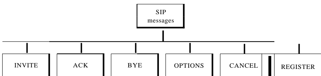
Figure 29.21 SIP messages
