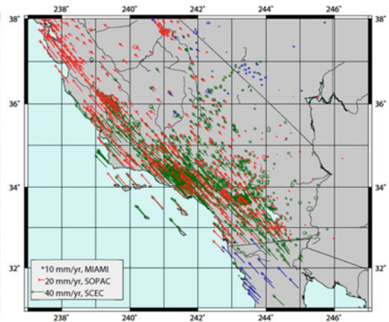
Fig. C.4 Plate tectonics at San Andreas Fault, California (Source: USGS)
