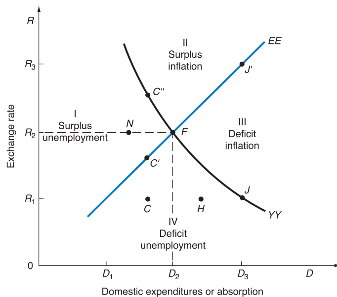
FIGURE 18.1. Swan Diagram.
