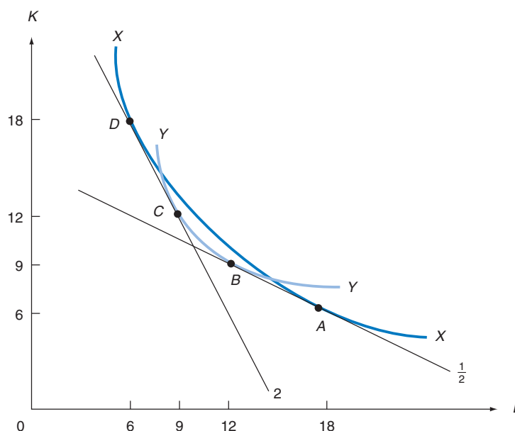
FIGURE 5.10. Factor-Intensity Reversal.
