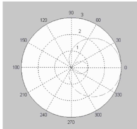
Figure 3-27 A polar plot of r = 1 + 2 \cos \theta
