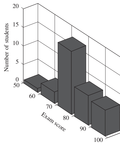
Figure 4-4 A three-dimensional bar chart
