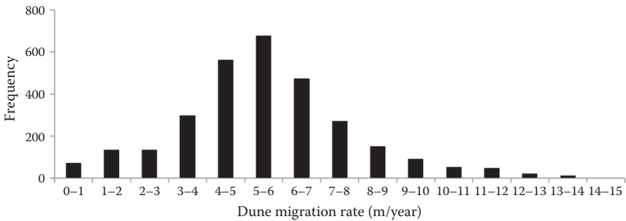
FIGURE 6.8 Histogram of dune migration rates (m year -1 ) for 3025 target points with source direction in the range of 225°–285°.
