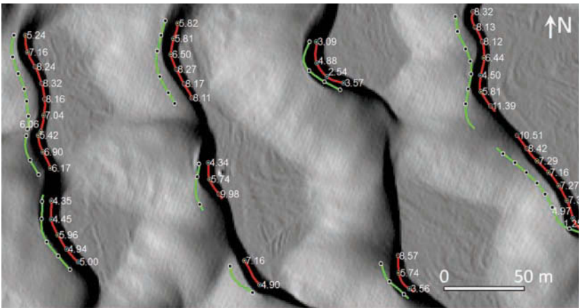
FIGURE 6.7 Sand dune migration rates (m year -1 ) displayed as labels for target points for the small area in Figure 6.5. Source lines (green), target lines (red), and pairs of source and target points (black) are also shown with a background of a shaded DEM for June 6, 2010.
