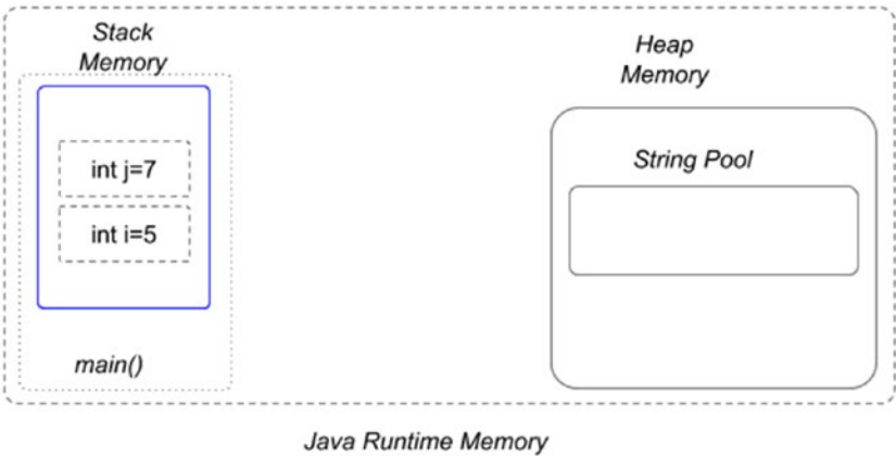
Figure 5-1. Java stack and heap memory, after declaring two primitive variables
