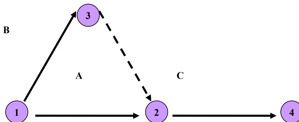
Figure 11: Dummy Activity
