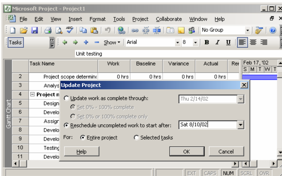
Figure 11.18: Rescheduling Tasks
