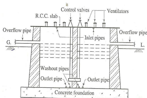
Surface reservoir
