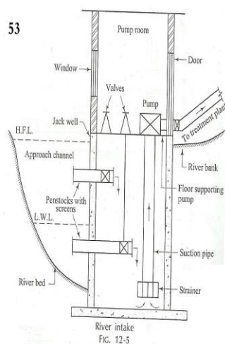
12-5. INTAKE TOWERS:
