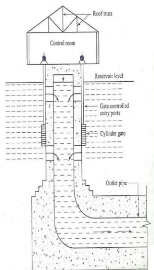
12-5. INTAKE TOWERS:
